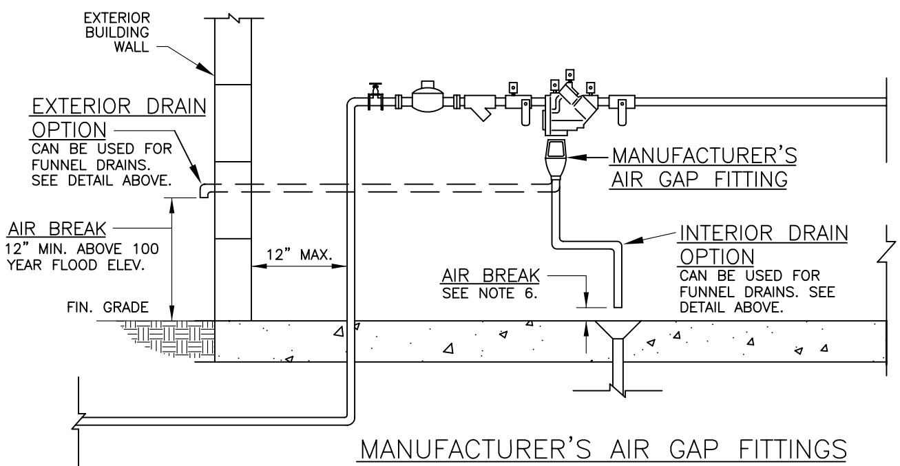
FUNNEL DRAIN
